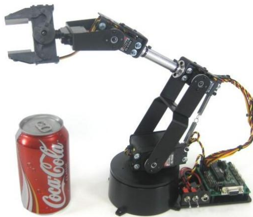
Figure 1.4 4 DOF Manipulator / arm robot from Lynxmotion suitable for education (source: lynxmotion.com).
